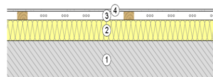
Figure 1: wall structure, including all layers
