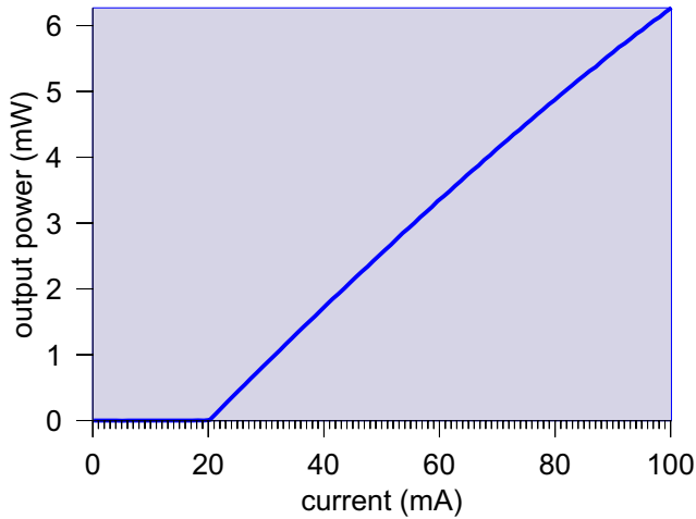
Current-Output-Power
