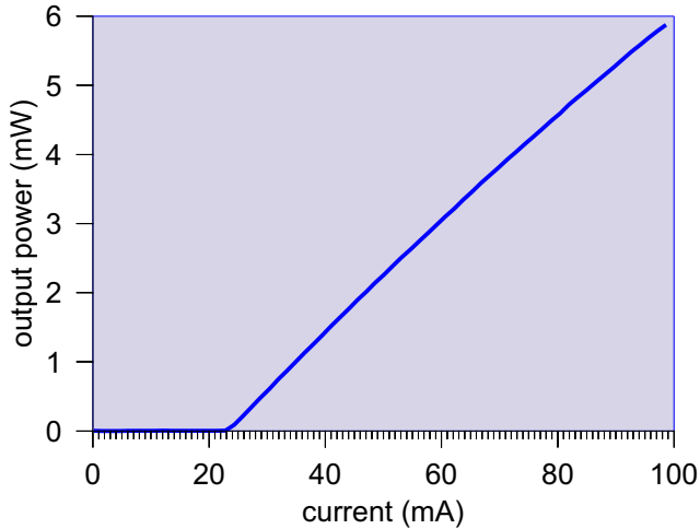
Current-Output-Power
