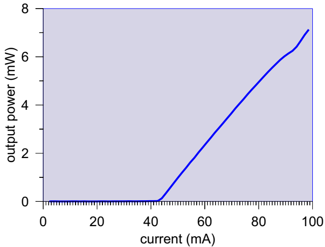
Current-Output-Power
