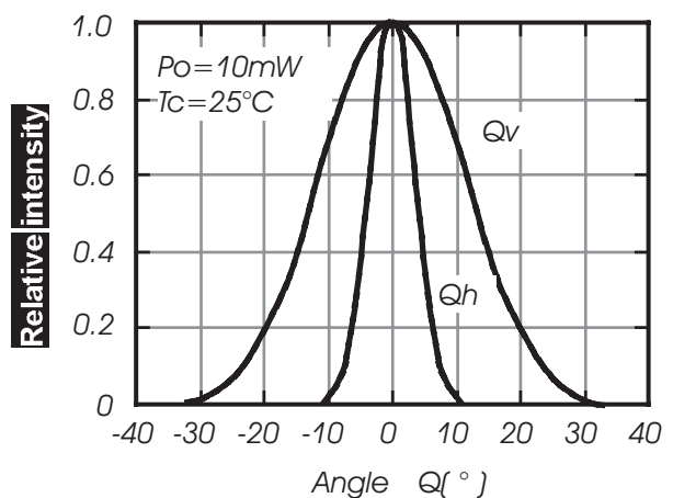
Beam divergence
