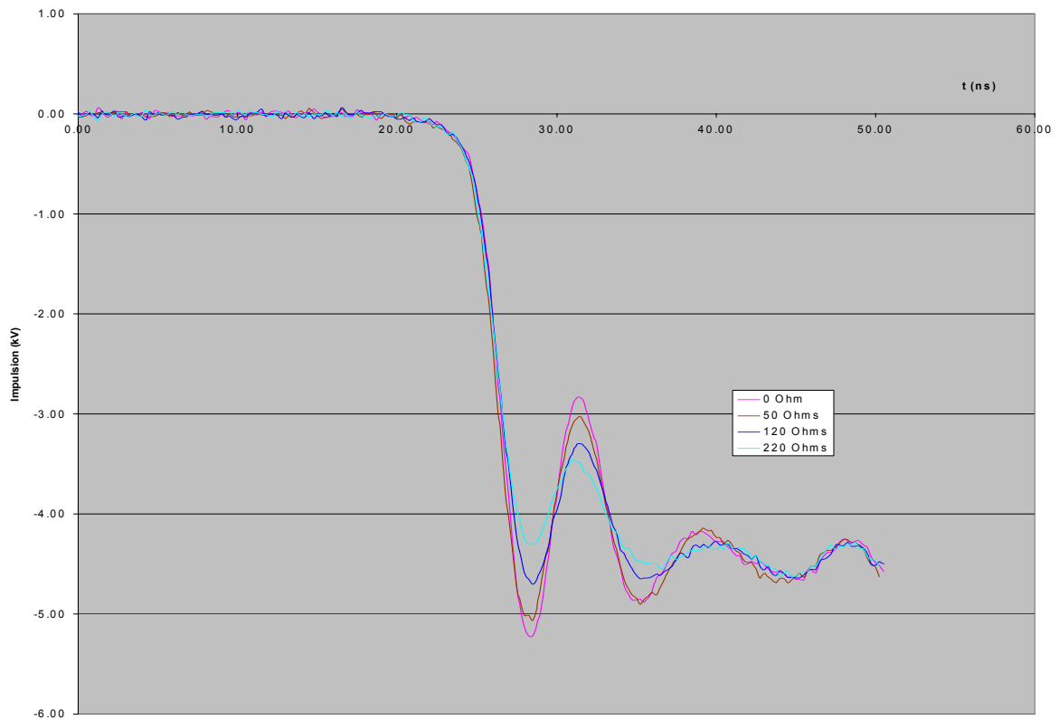
Fig.4 : a resistor in series with the Pockel's cell can smooth the rebound, test with several values of resistors
