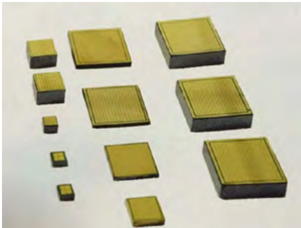
CZT high resolution pixel detector
