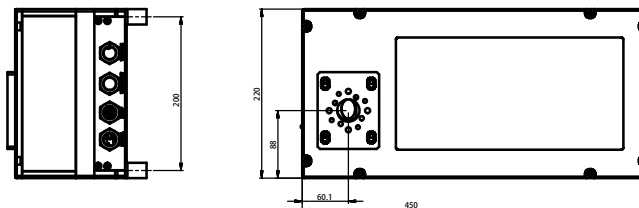
HQF-1064/532-5-500-400/200-P
