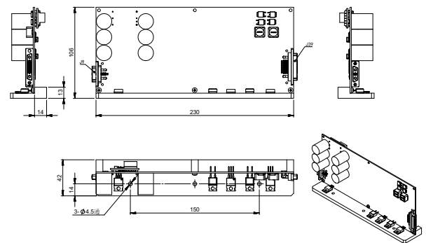
Drive Board
