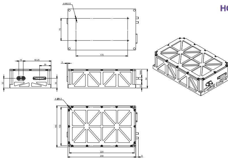
Laser Head
