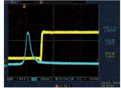
Photodiode output signal
