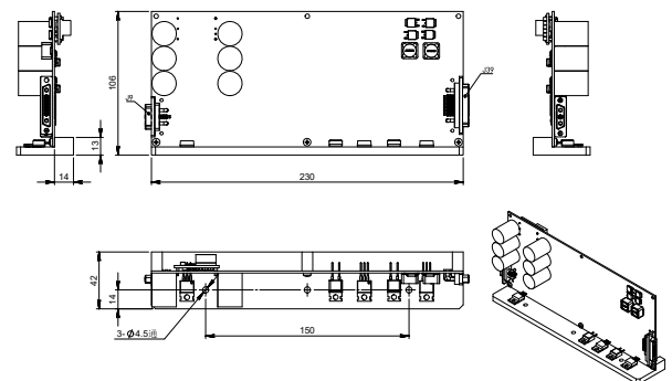
Drive Board
