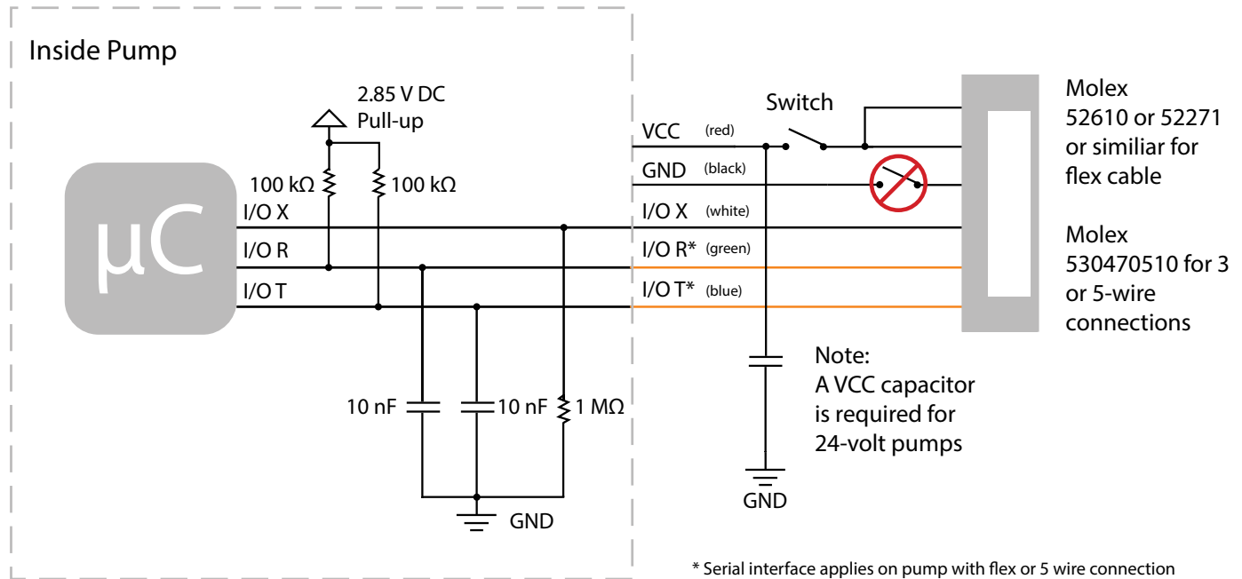
Figure 2: Electronic interface
